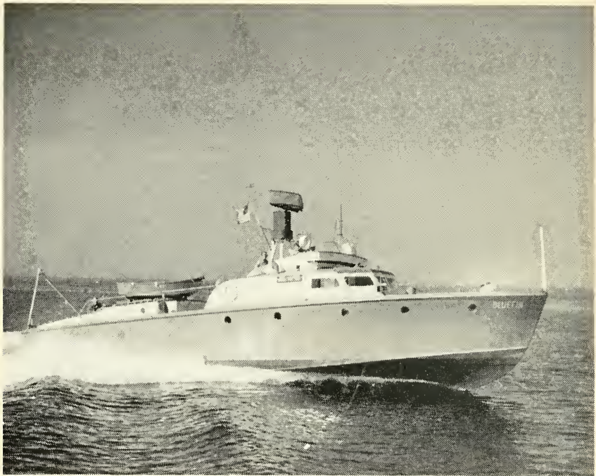
FIGURE 20. 63-foot Fish and Game patrol boat BLUEFIN. The commission operates two of these vessels in Southern California waters. Equipped with two 630-h.p. Hall Scott Defender engines, radar, radio and full marine equipment. Photograph by Vernon M. Haden, San Pedro.
